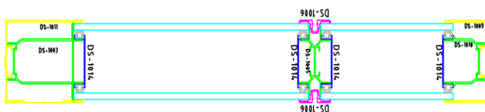
SECTION - A
