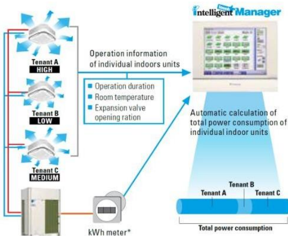
Fig 1. Power Proportional Distribution concept
