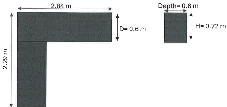
Top View of Bottom Cabinet
