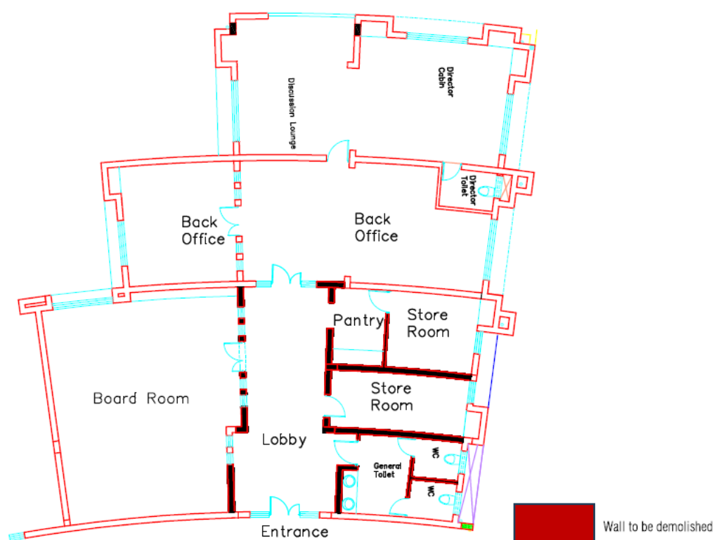
Existing Layout of Director's Secretariat
