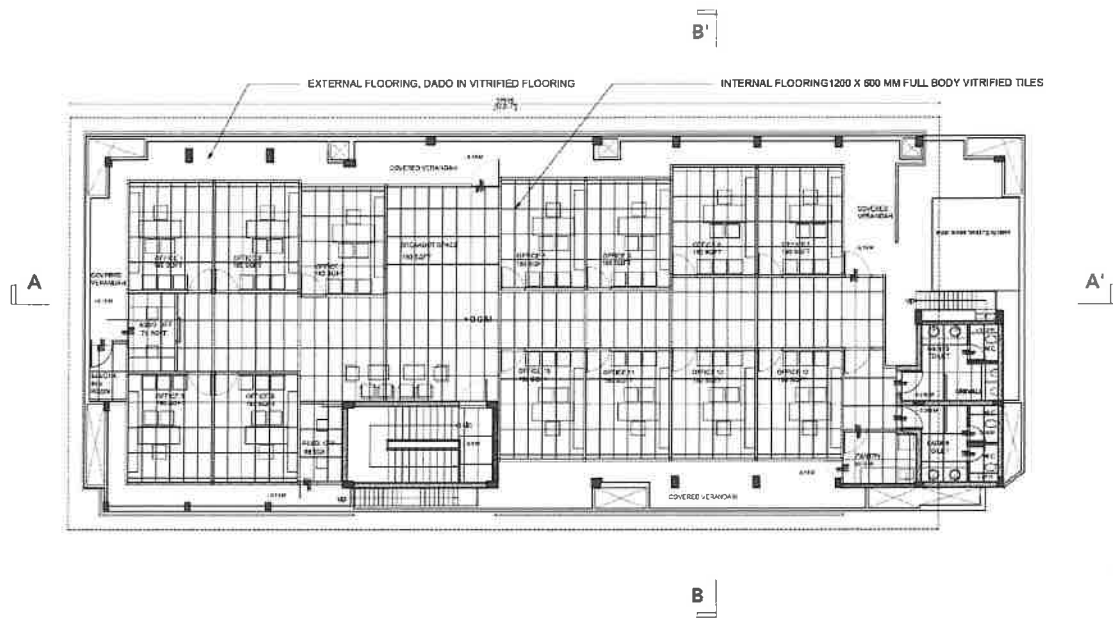
FLOORING PLAN
