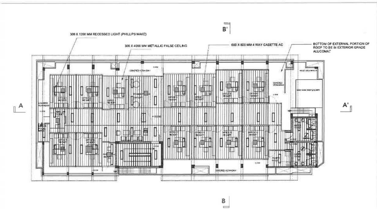
FALSE CEILING PLAN WITH LIGHTING AND AC LAYOUT
