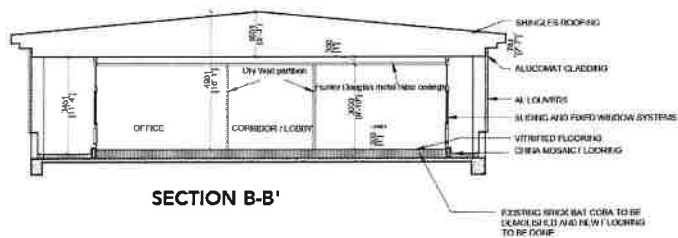
SCHEMATIC SECTIONS
