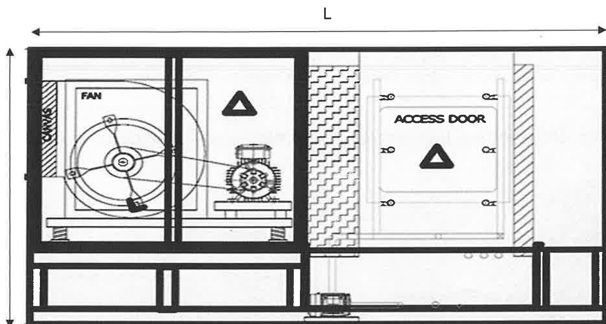
SIDE VIEW
